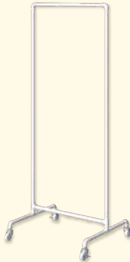
Gas white S-Rack W600 W600×D500×H1350 91856
