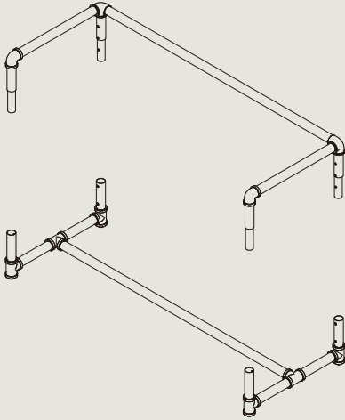
ANGLE FRAME W1200×D467 91501
